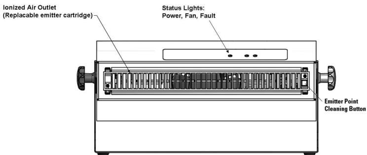
Figure 2. Aerostat XC2 Front-panel
